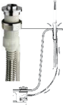
Bath Rim Shower Socket With Draining System | PD467
